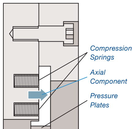
Figure 2. LF Vent Pac Assembly
